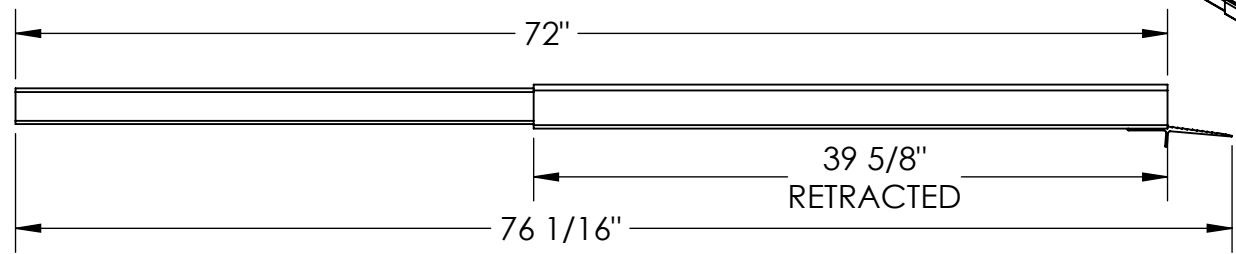
OUTER RAMP DETAIL SCALE 1:4
