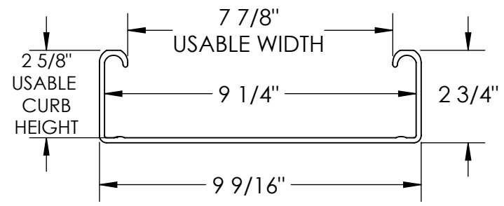
OUTER RAMP DETAIL SCALE 1:4
